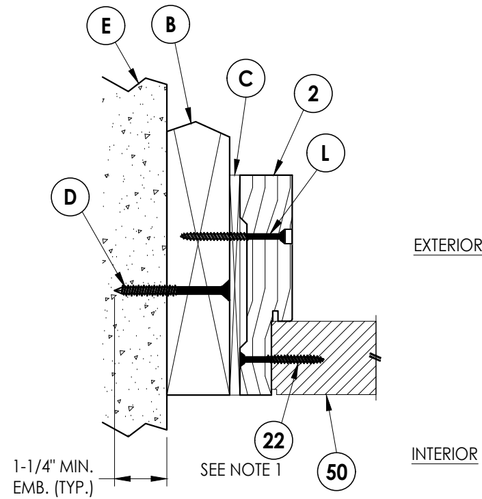
3 HORIZONTAL CROSS SECTION 5 Shown w/ 2X Buck Inswing shown (Outswing similar)
