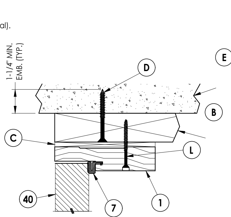
2 VERTICAL CROSS SECTION 5 Shown w/ 2X Buck Inswing shown (Outswing similar)
