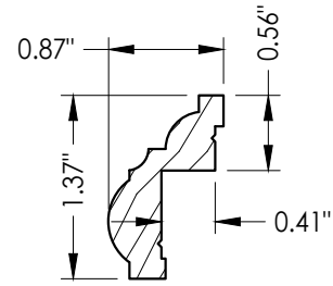
GLAZING BEAD
